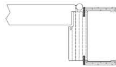
stipite standard cornice standard
